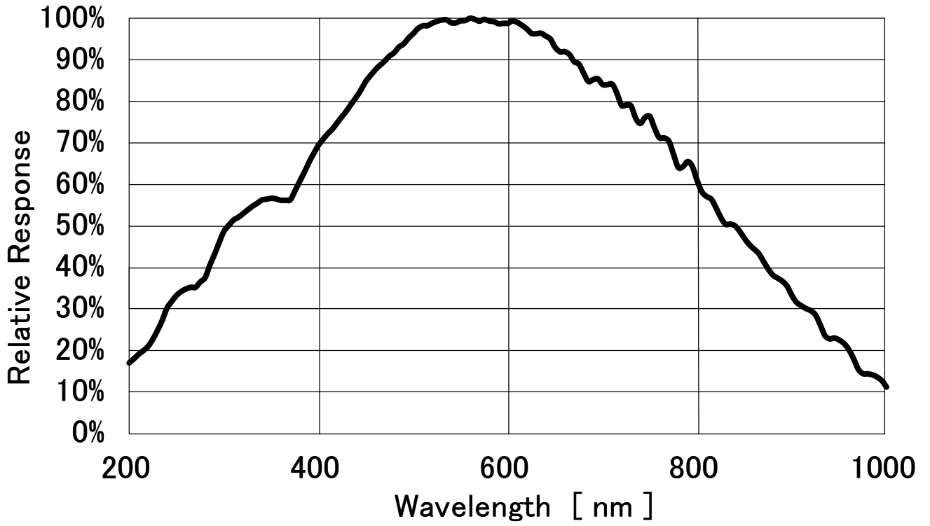
Spectral sensitivity characteristics
